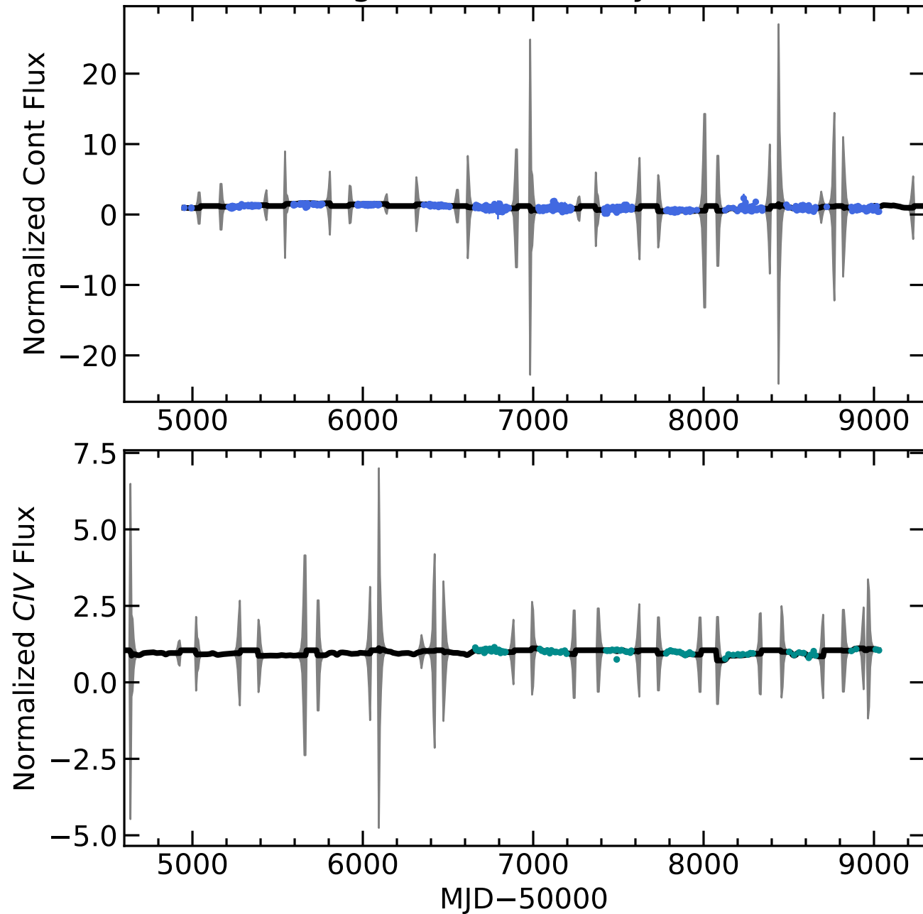
RM208 Light Curves (w/ PyROA model)
