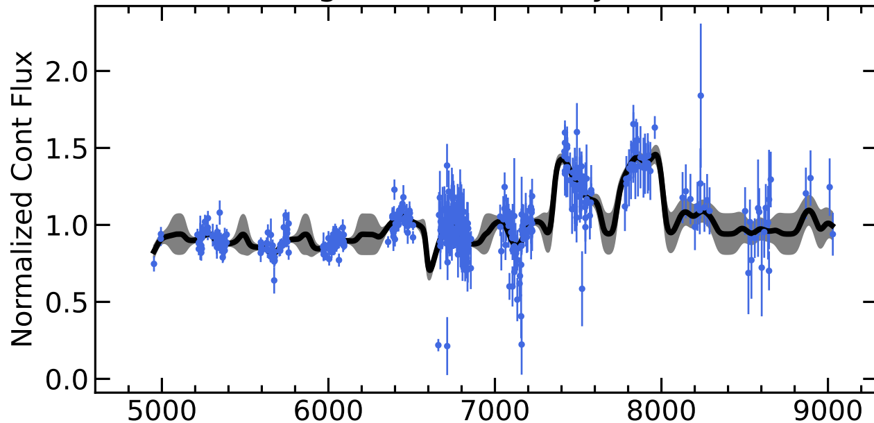
RM209 Light Curves (w/ PyROA model)
