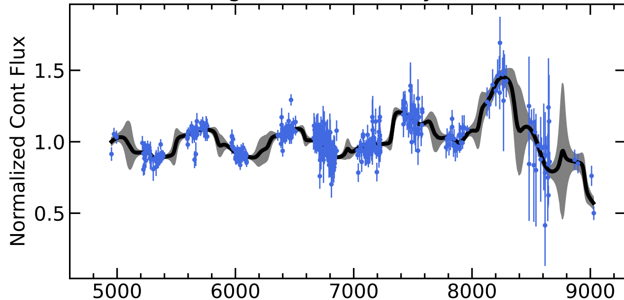
RM210 Light Curves (w/ PyROA model)
