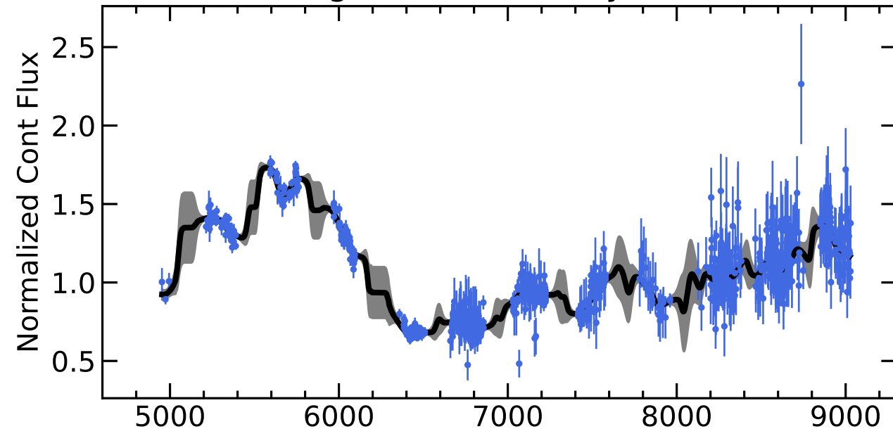
RM212 Light Curves (w/ PyROA model)
