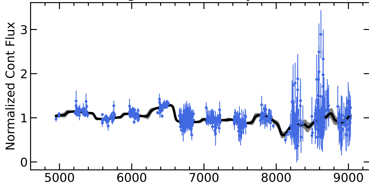
RM213 Light Curves (w/ PyROA model)
