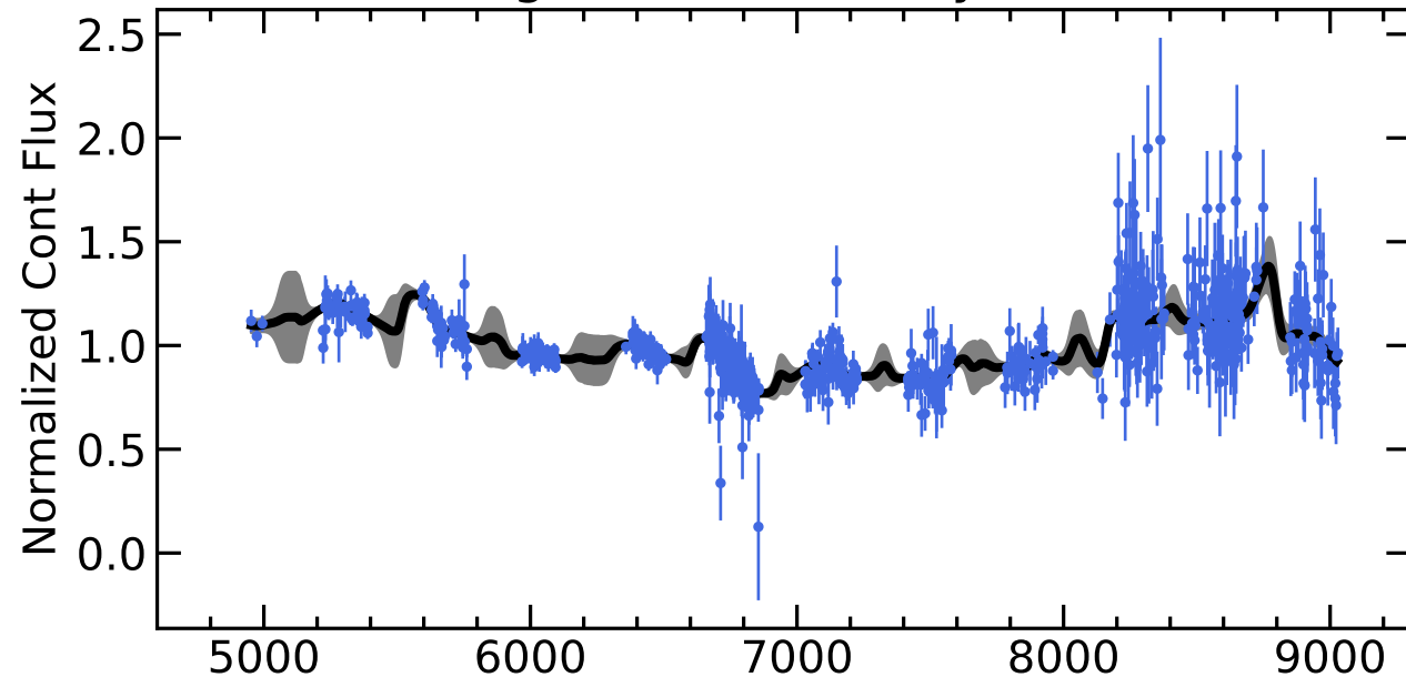
RM214 Light Curves (w/ PyROA model)
