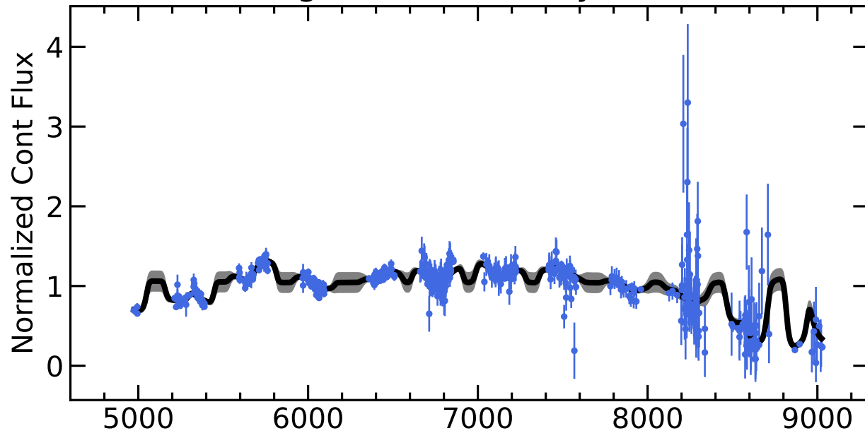
RM216 Light Curves (w/ PyROA model)
