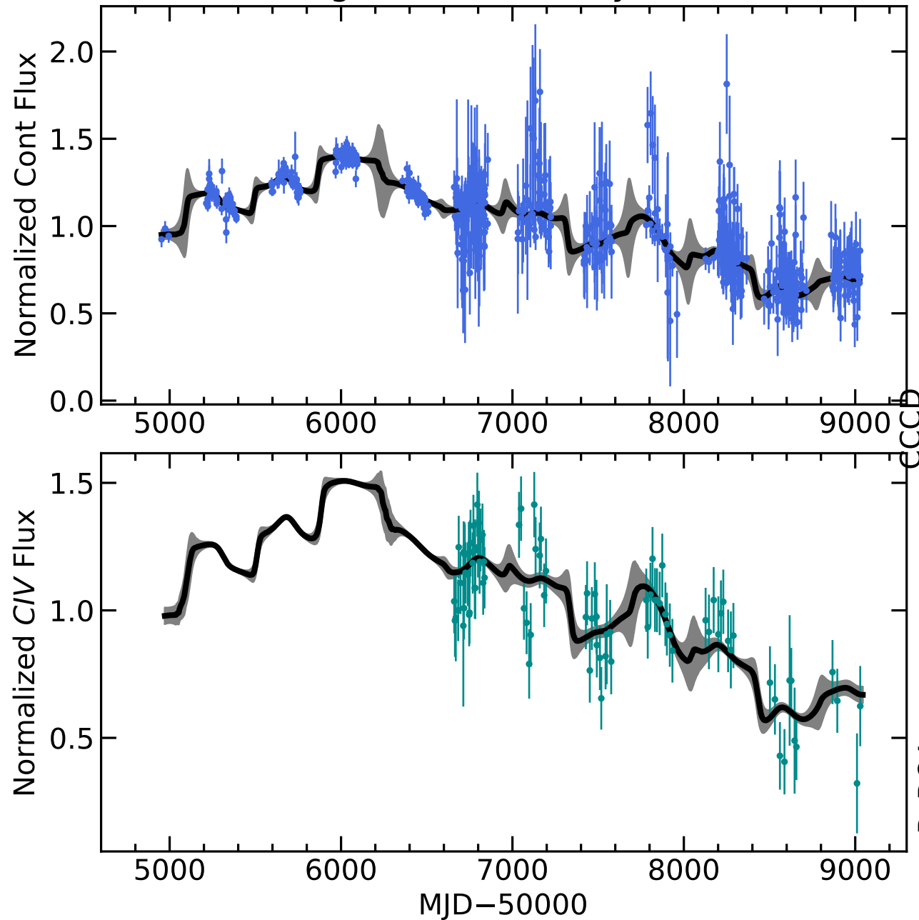
RM217 Light Curves (w/ PyROA model)
