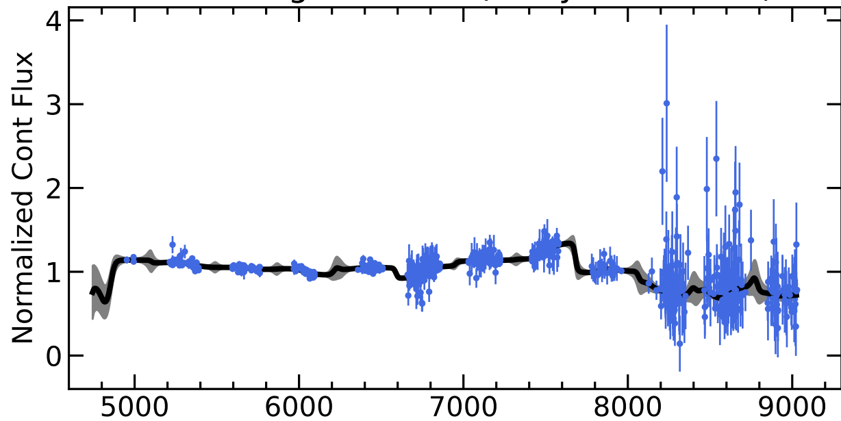
RM218 Light Curves (w/ PyROA model)
