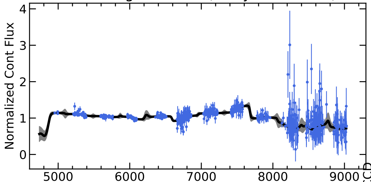
RM218 Light Curves (w/ PyROA model)
