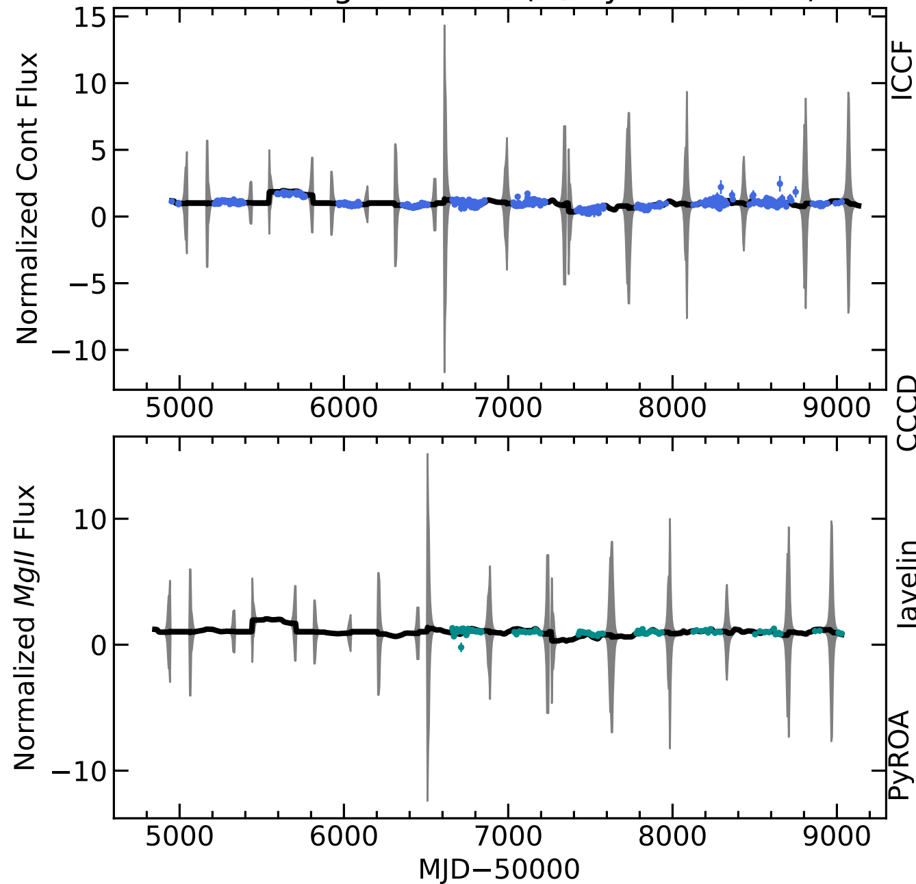
RM219 Light Curves (w/ PyROA model)
