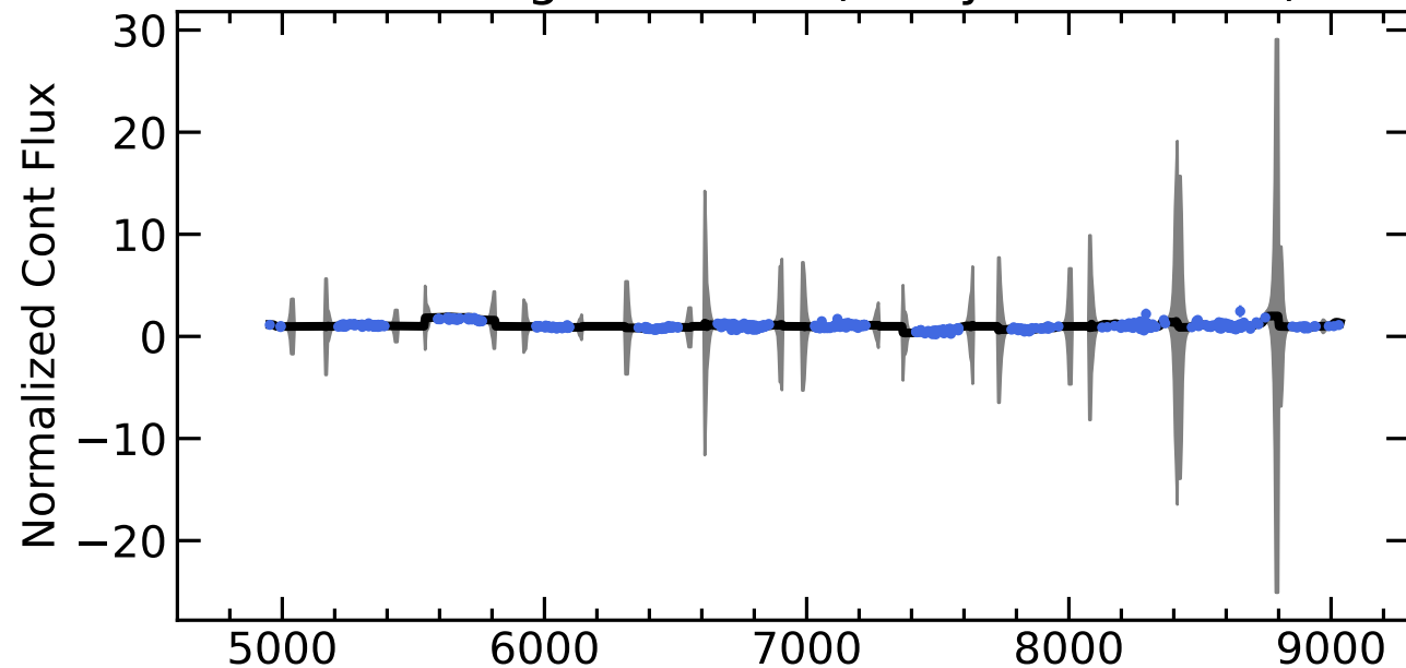
RM219 Light Curves (w/ PyROA model)
