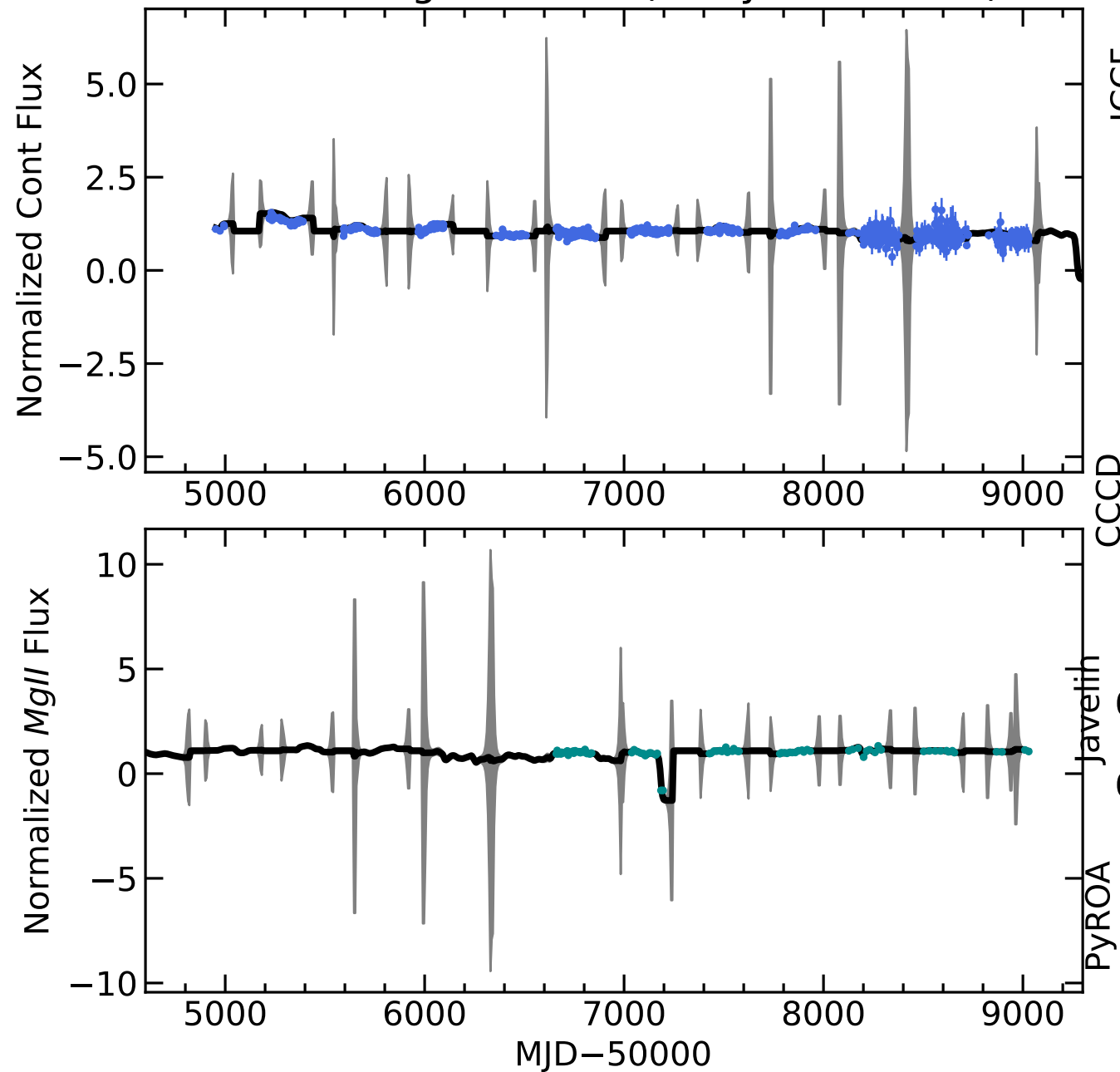
RM220 Light Curves (w/ PyROA model)
