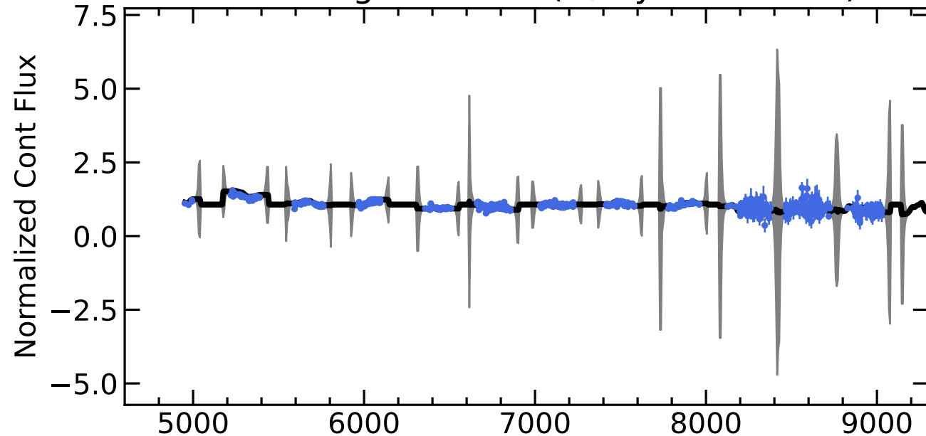
RM220 Light Curves (w/ PyROA model)
