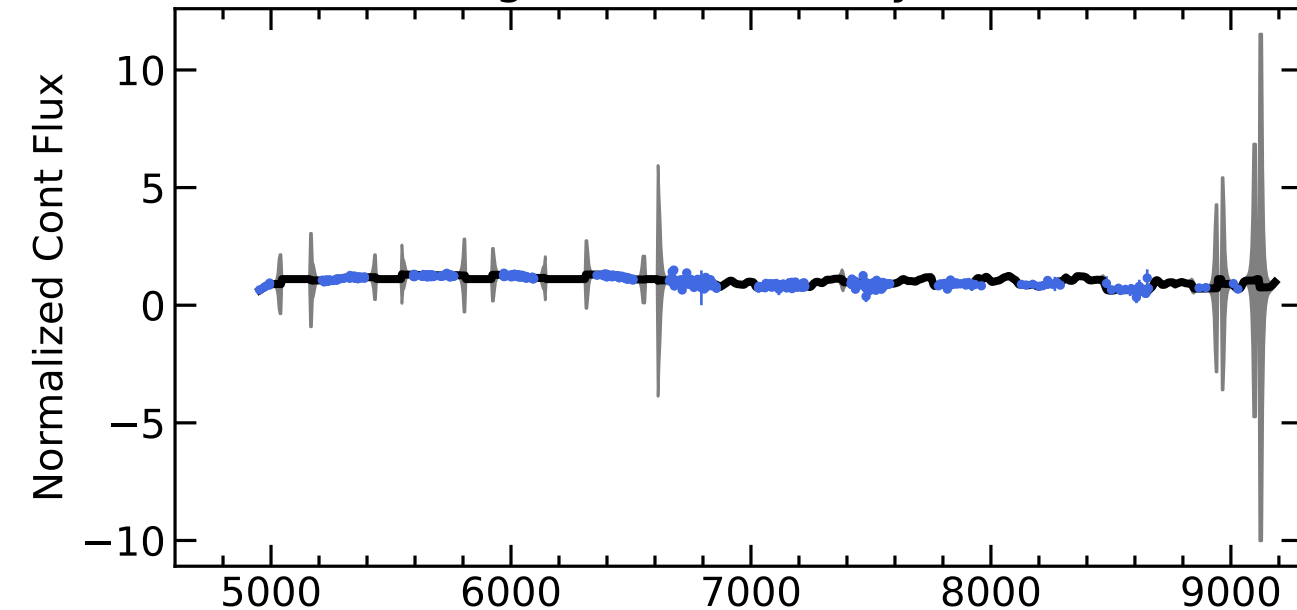
RM221 Light Curves (w/ PyROA model)
