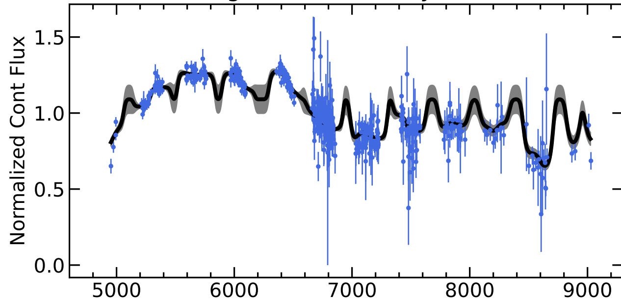
RM221 Light Curves (w/ PyROA model)
