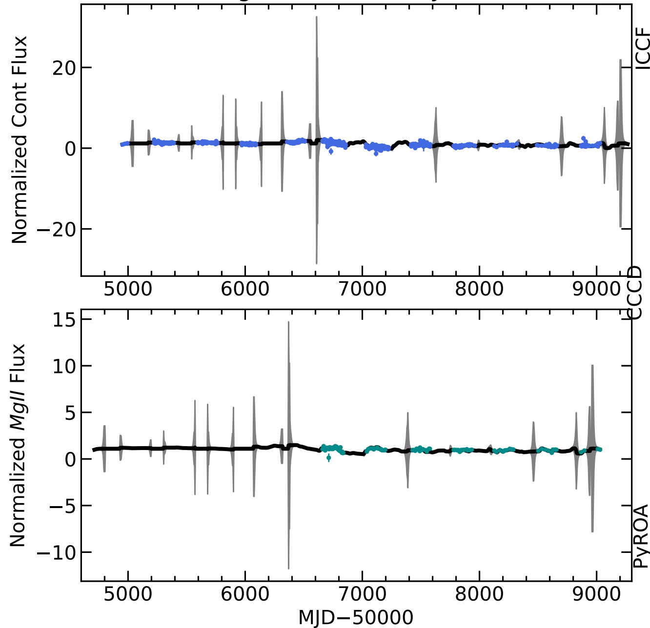
RM222 Light Curves (w/ PyROA model)
