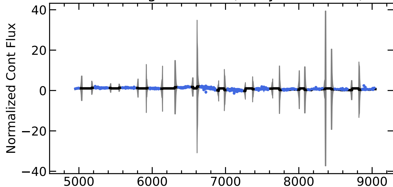
RM222 Light Curves (w/ PyROA model)
