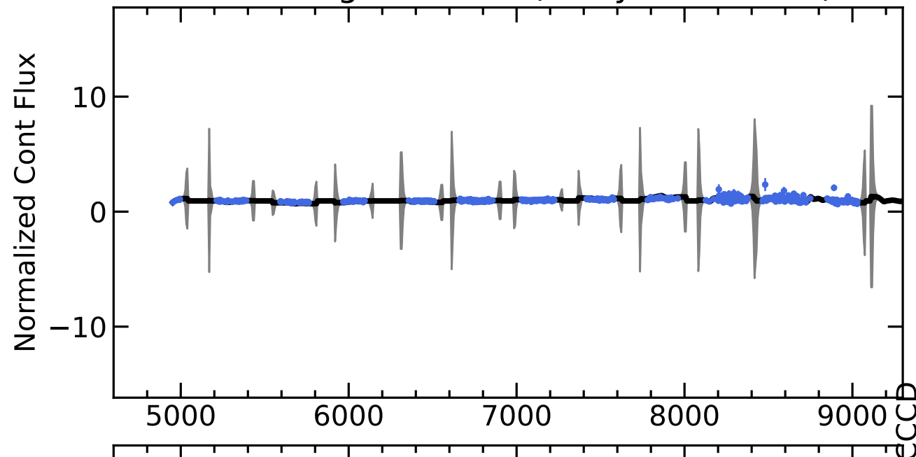
RM223 Light Curves (w/ PyROA model)
