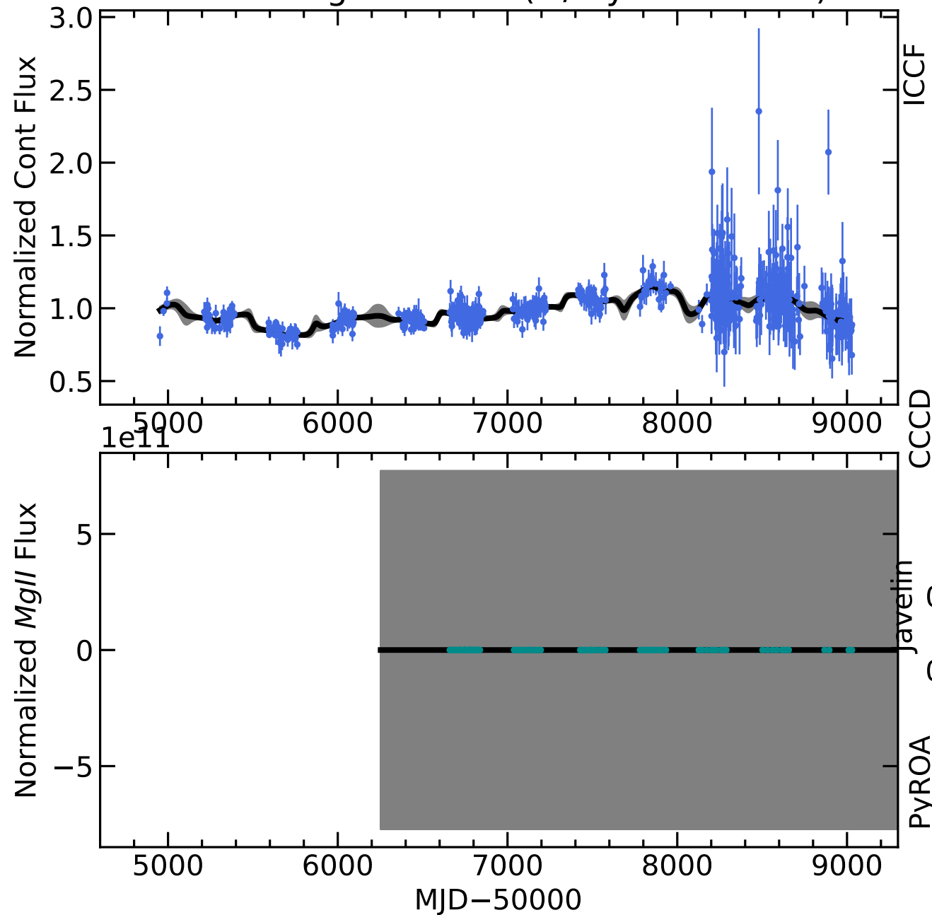
RM223 Light Curves (w/ PyROA model)
