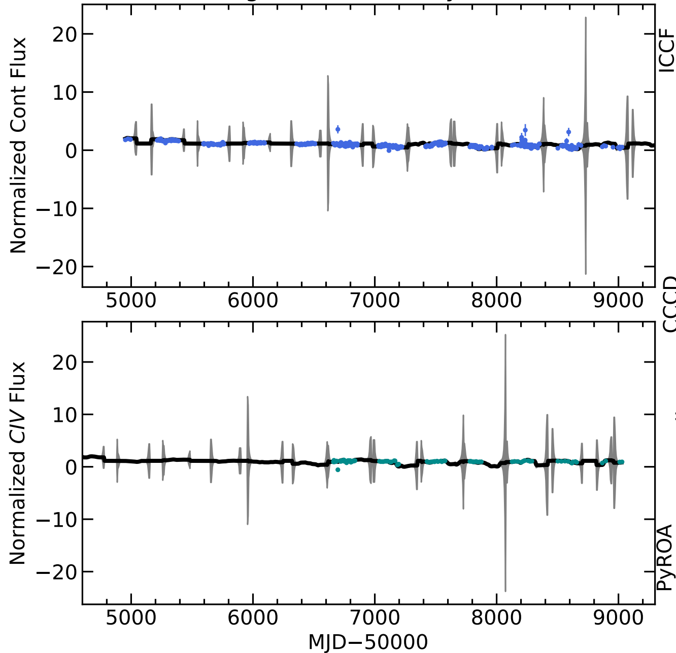
RM225 Light Curves (w/ PyROA model)
