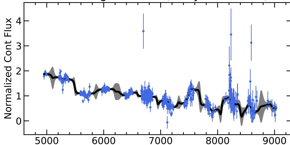
RM225 Light Curves (w/ PyROA model)
