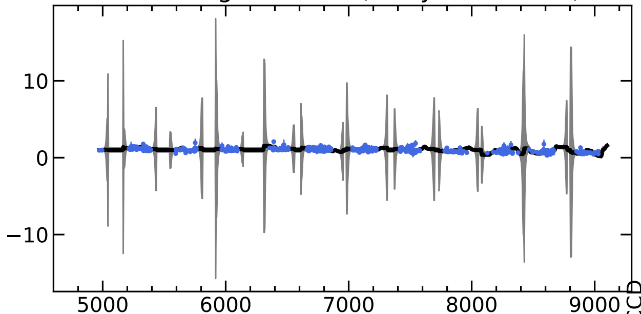
RM226 Light Curves (w/ PyROA model)
