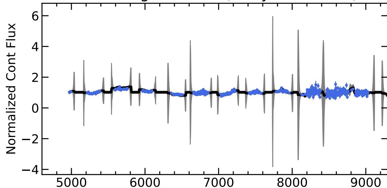
RM227 Light Curves (w/ PyROA model)
