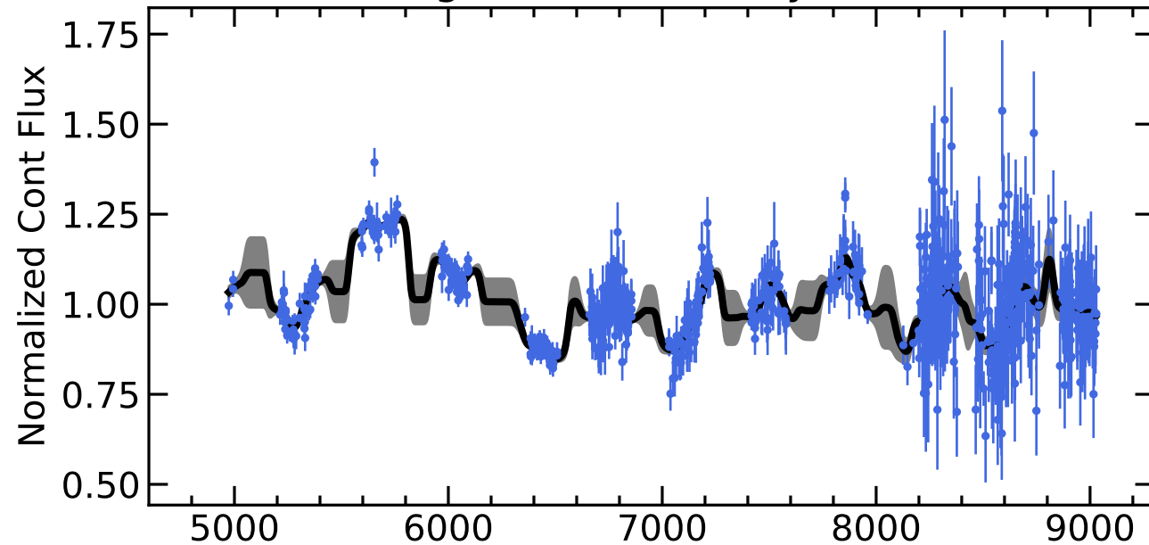
RM227 Light Curves (w/ PyROA model)
