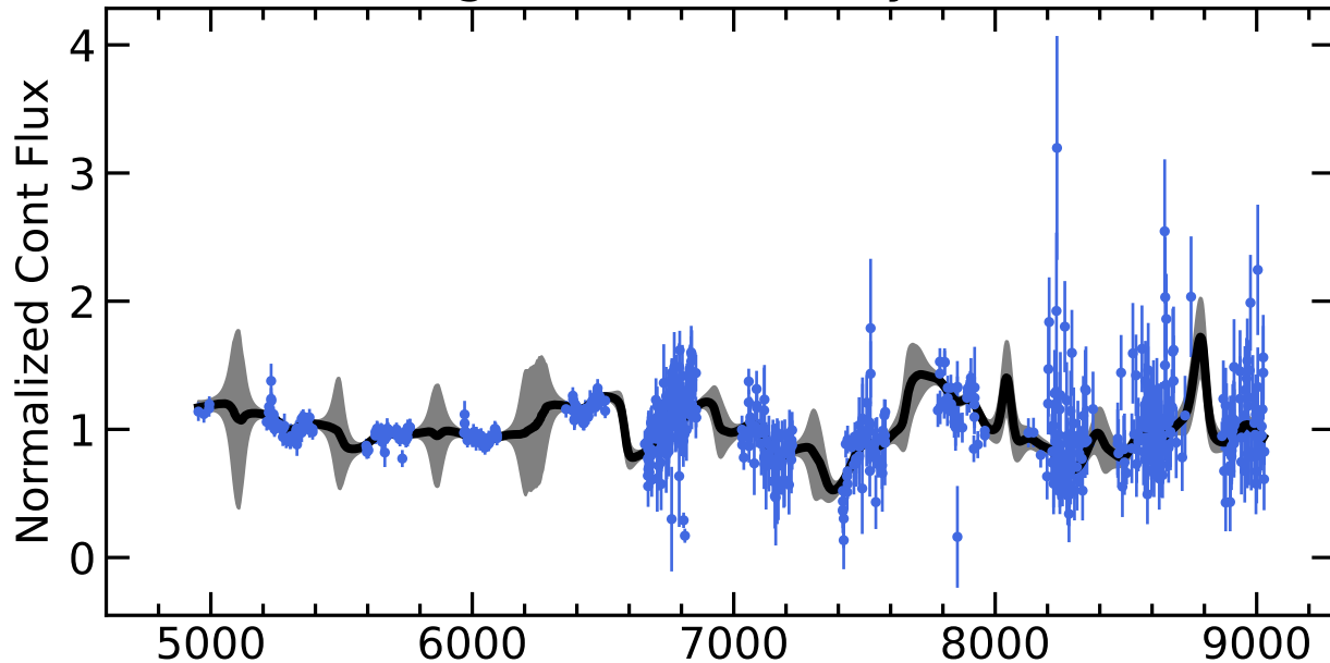
RM228 Light Curves (w/ PyROA model)
