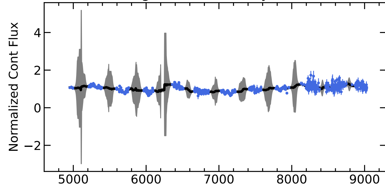
RM229 Light Curves (w/ PyROA model)
