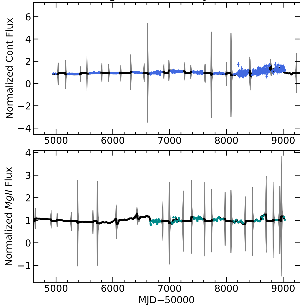
RM230 Light Curves (w/ PyROA model)
