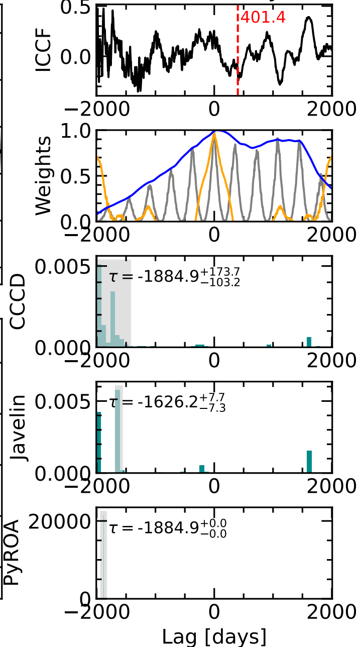
Time Delay
