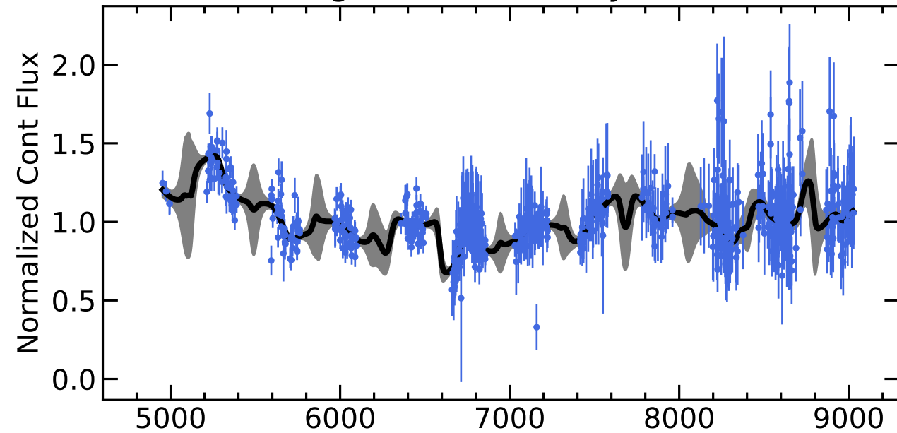
RM232 Light Curves (w/ PyROA model)
