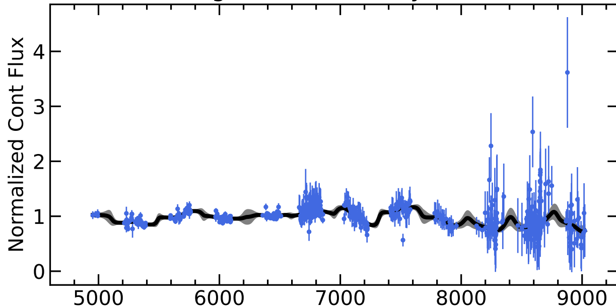
RM234 Light Curves (w/ PyROA model)
