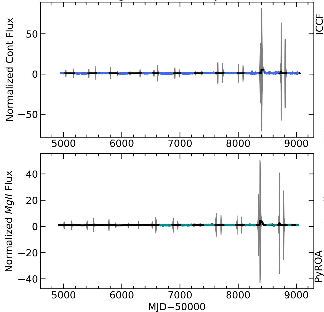
RM236 Light Curves (w/ PyROA model)
