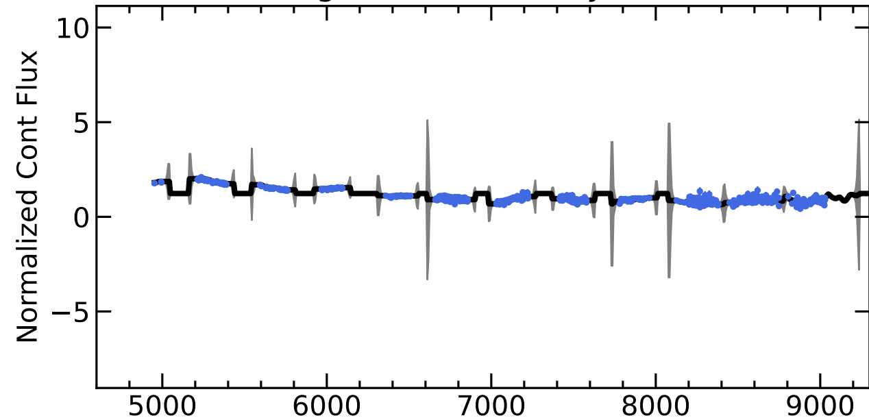
RM237 Light Curves (w/ PyROA model)
