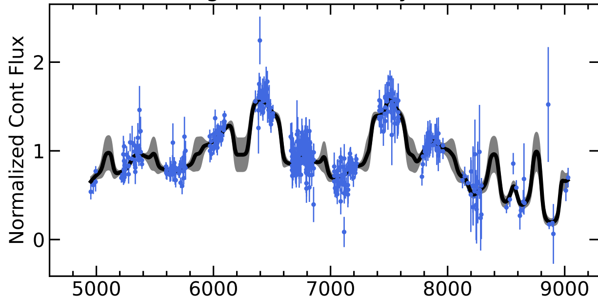
RM239 Light Curves (w/ PyROA model)
