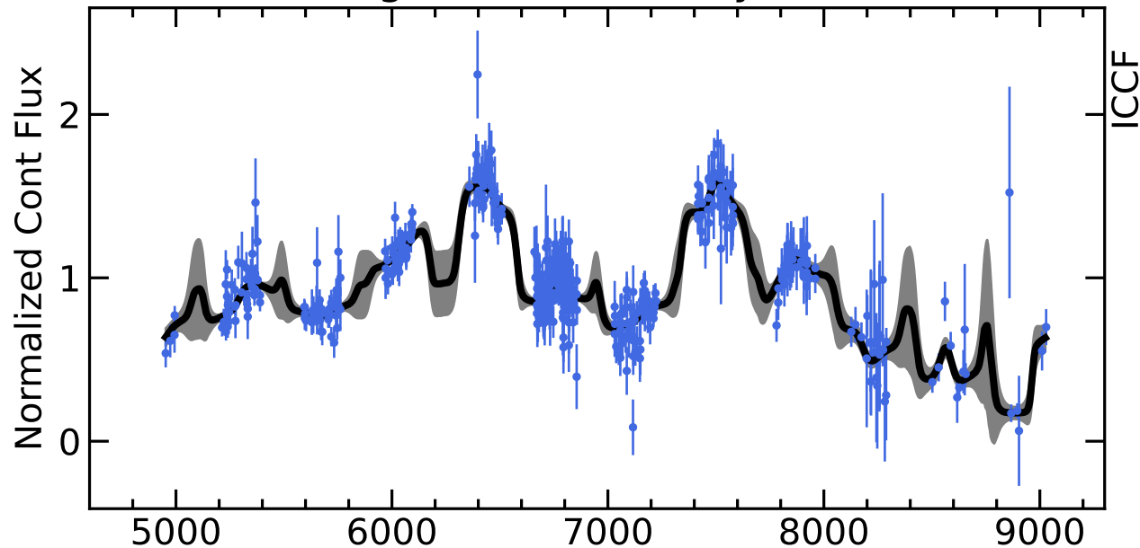
RM239 Light Curves (w/ PyROA model)
