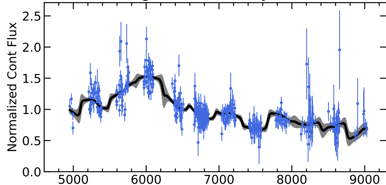
RM240 Light Curves (w/ PyROA model)
