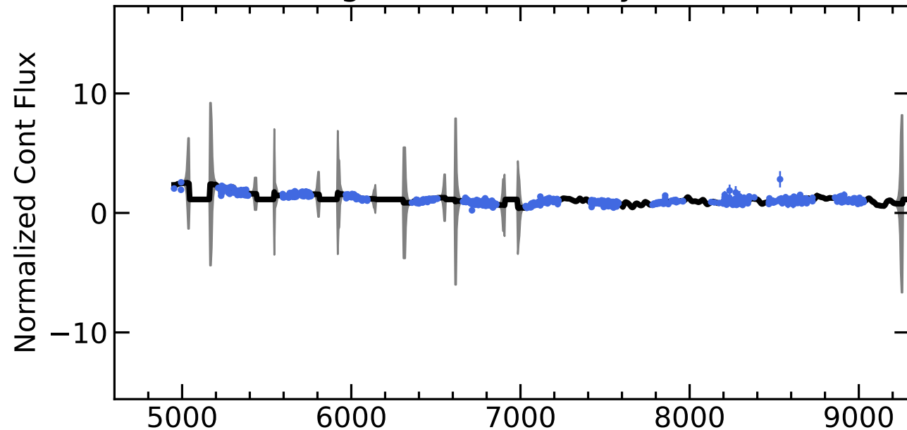
RM241 Light Curves (w/ PyROA model)
