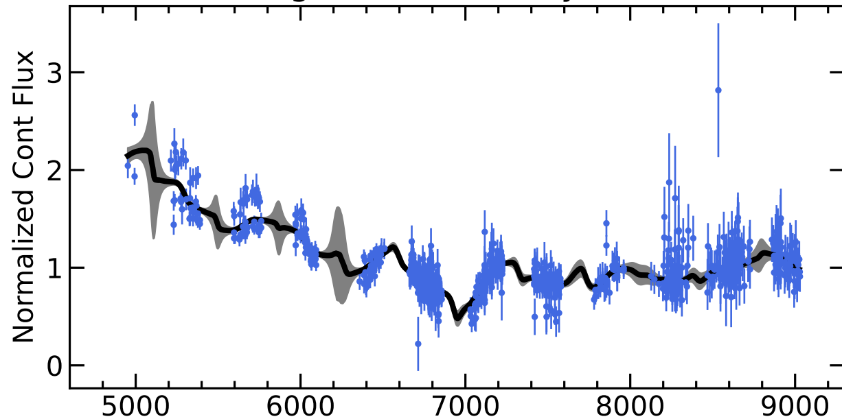
RM241 Light Curves (w/ PyROA model)
