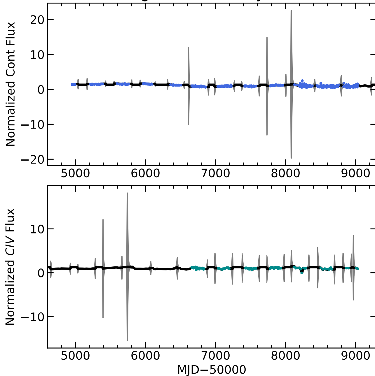
RM242 Light Curves (w/ PyROA model)
