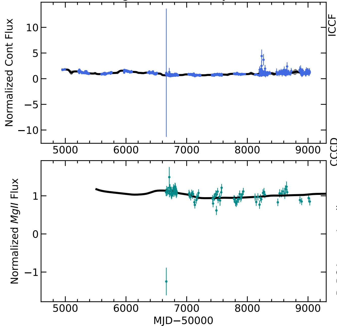
RM244 Light Curves (w/ PyROA model)
