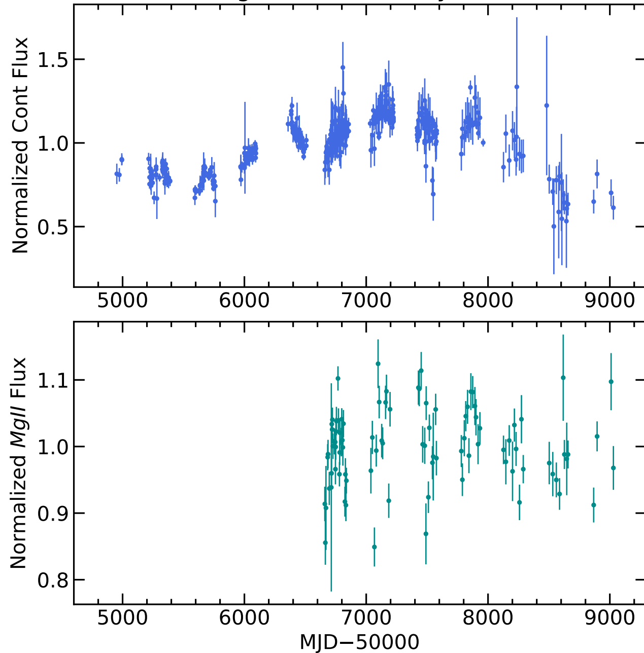
RM245 Light Curves (w/ PyROA model)
