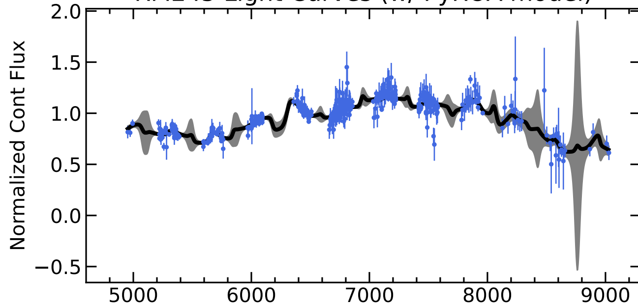
RM245 Light Curves (w/ PyROA model)
