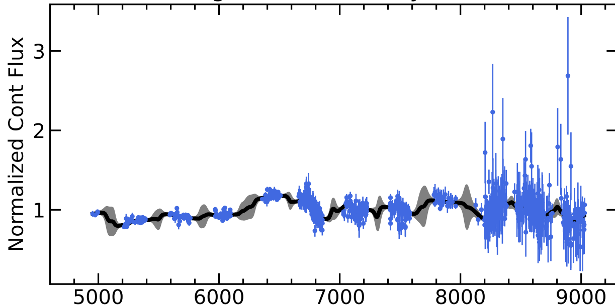
RM246 Light Curves (w/ PyROA model)
