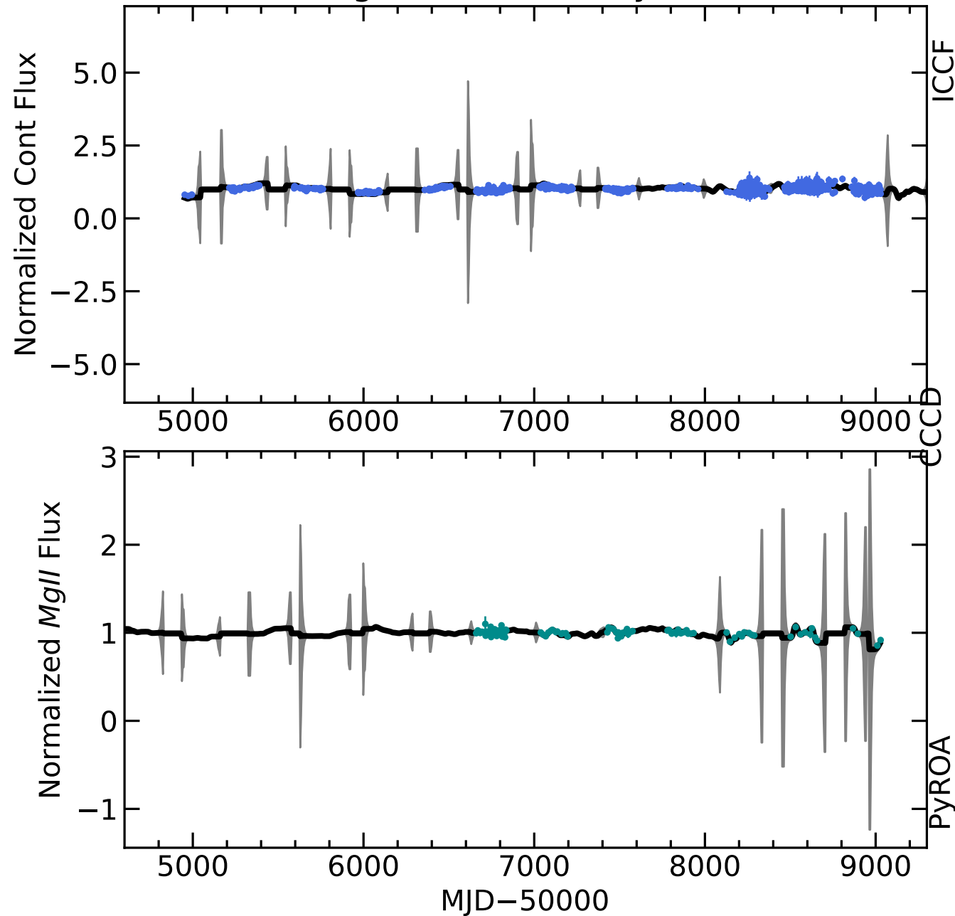
RM247 Light Curves (w/ PyROA model)
