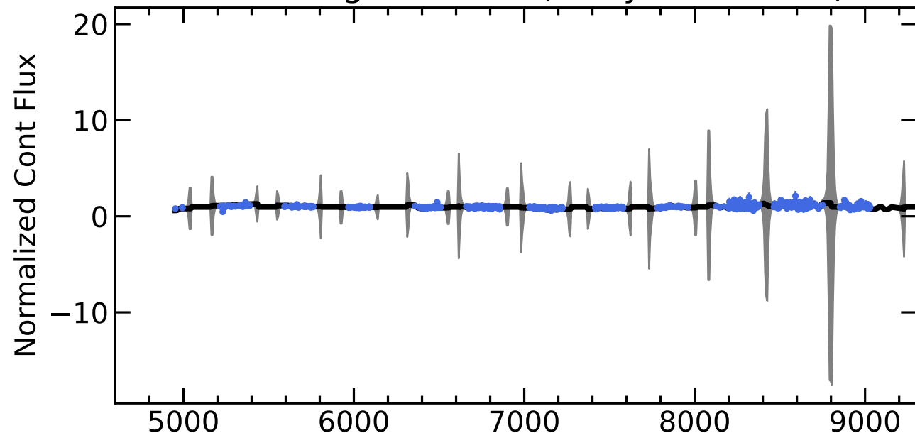
RM248 Light Curves (w/ PyROA model)
