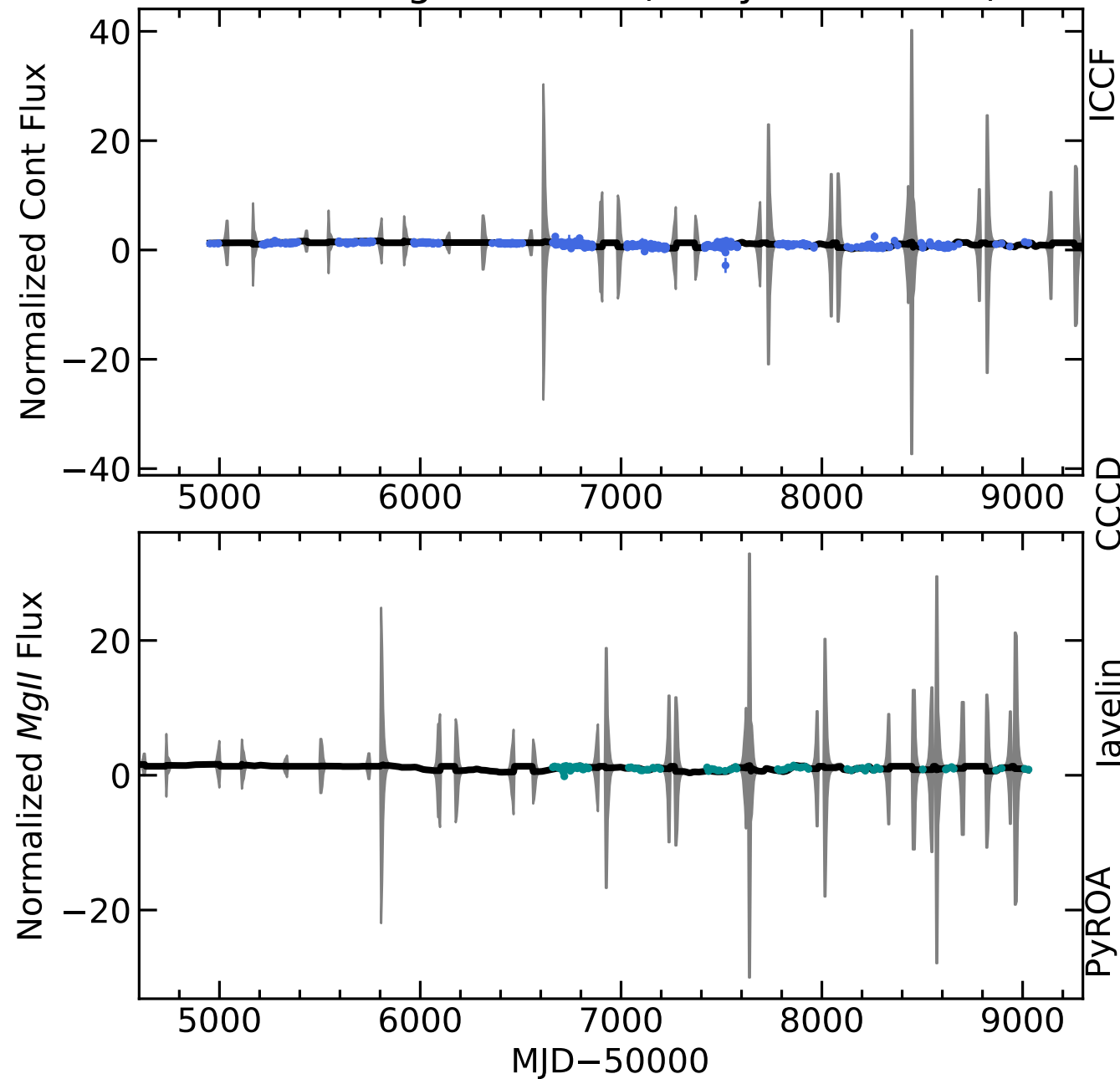
RM249 Light Curves (w/ PyROA model)
