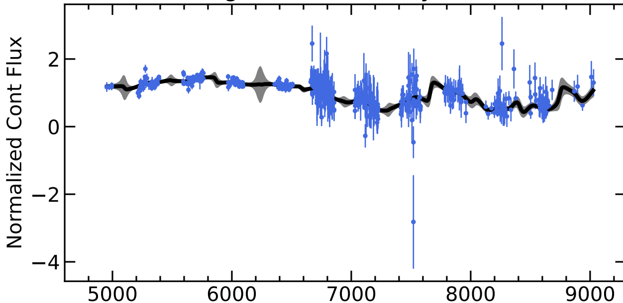
RM249 Light Curves (w/ PyROA model)
