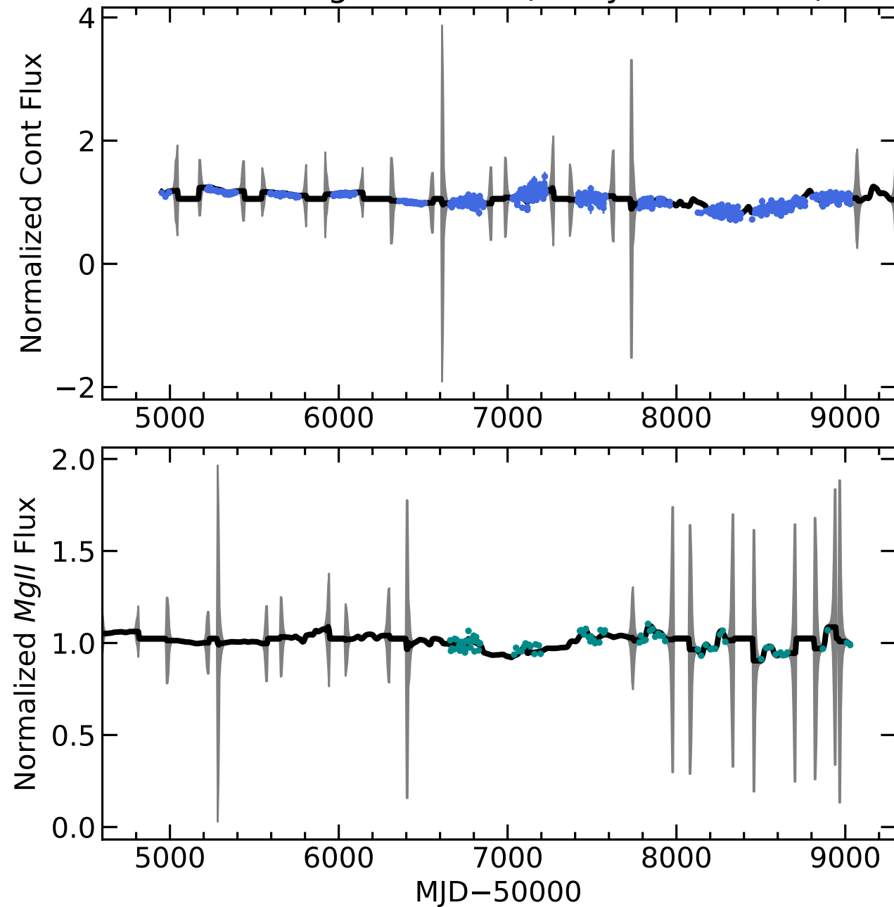
RM250 Light Curves (w/ PyROA model)
