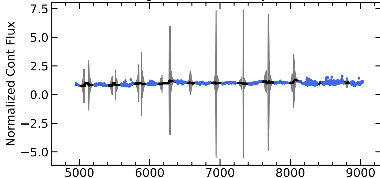
RM252 Light Curves (w/ PyROA model)
