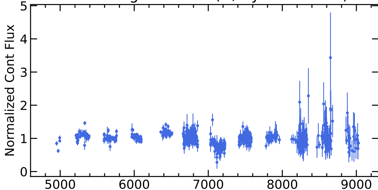
RM254 Light Curves (w/ PyROA model)
