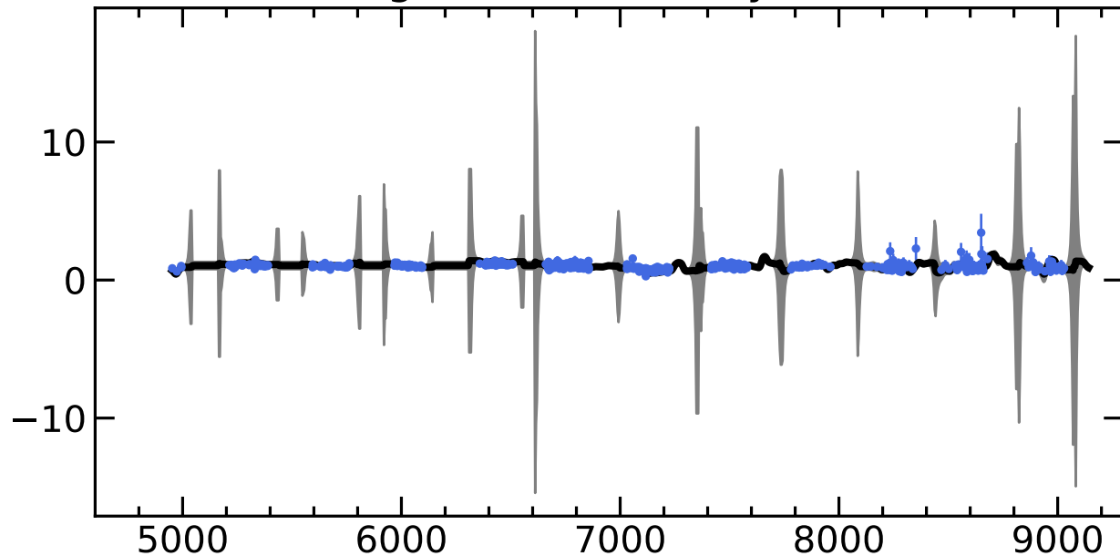
RM254 Light Curves (w/ PyROA model)
