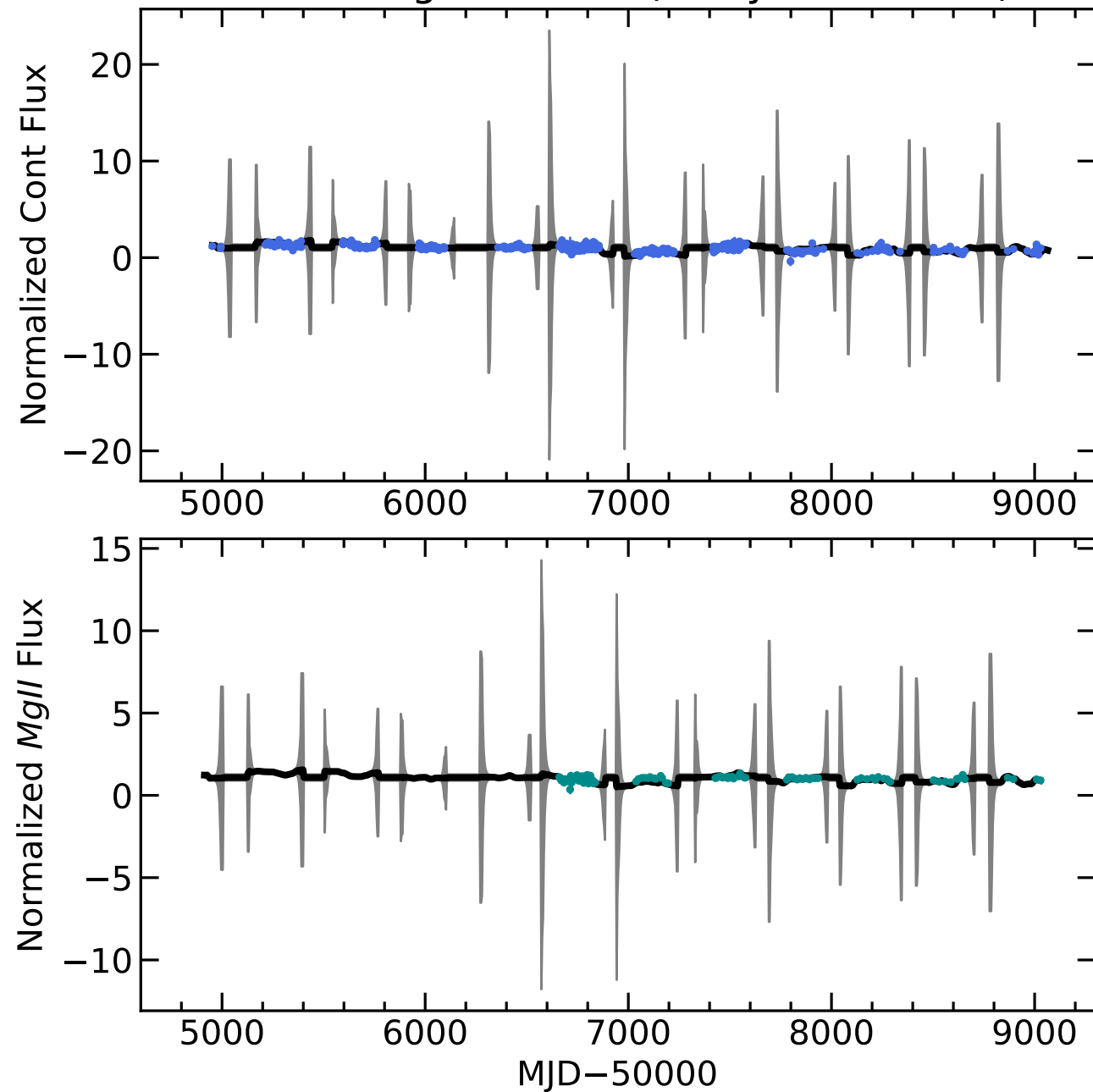
RM255 Light Curves (w/ PyROA model)
