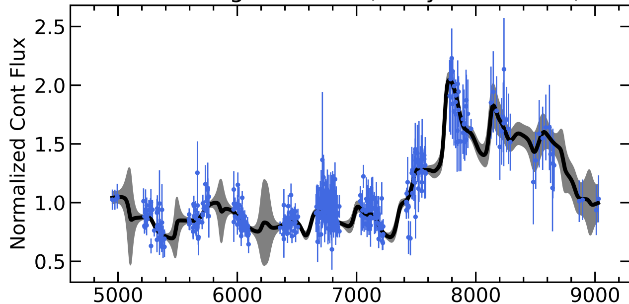
RM256 Light Curves (w/ PyROA model)
