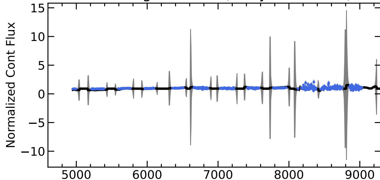
RM257 Light Curves (w/ PyROA model)
