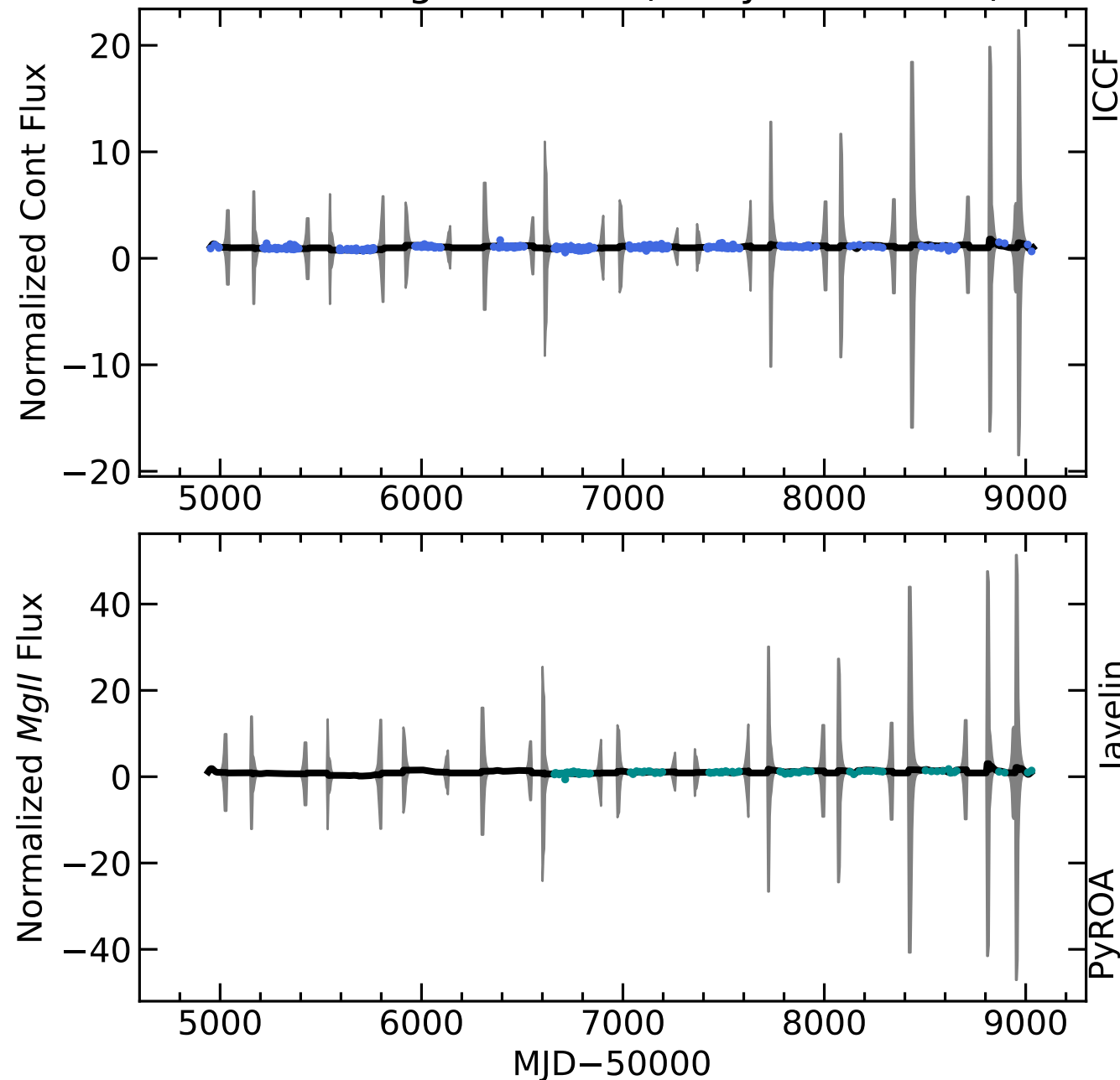
RM258 Light Curves (w/ PyROA model)
