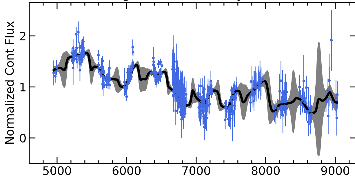
RM259 Light Curves (w/ PyROA model)
