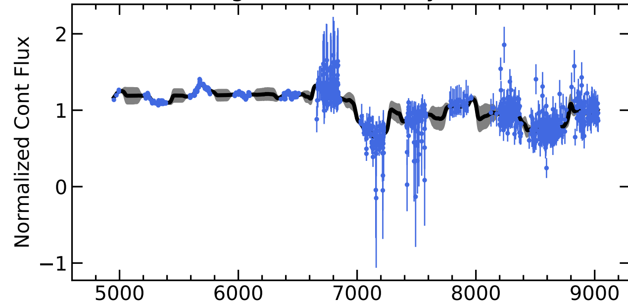
RM260 Light Curves (w/ PyROA model)
