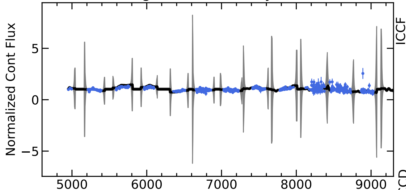
RM261 Light Curves (w/ PyROA model)
