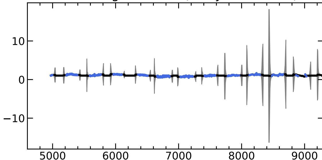
RM263 Light Curves (w/ PyROA model)
