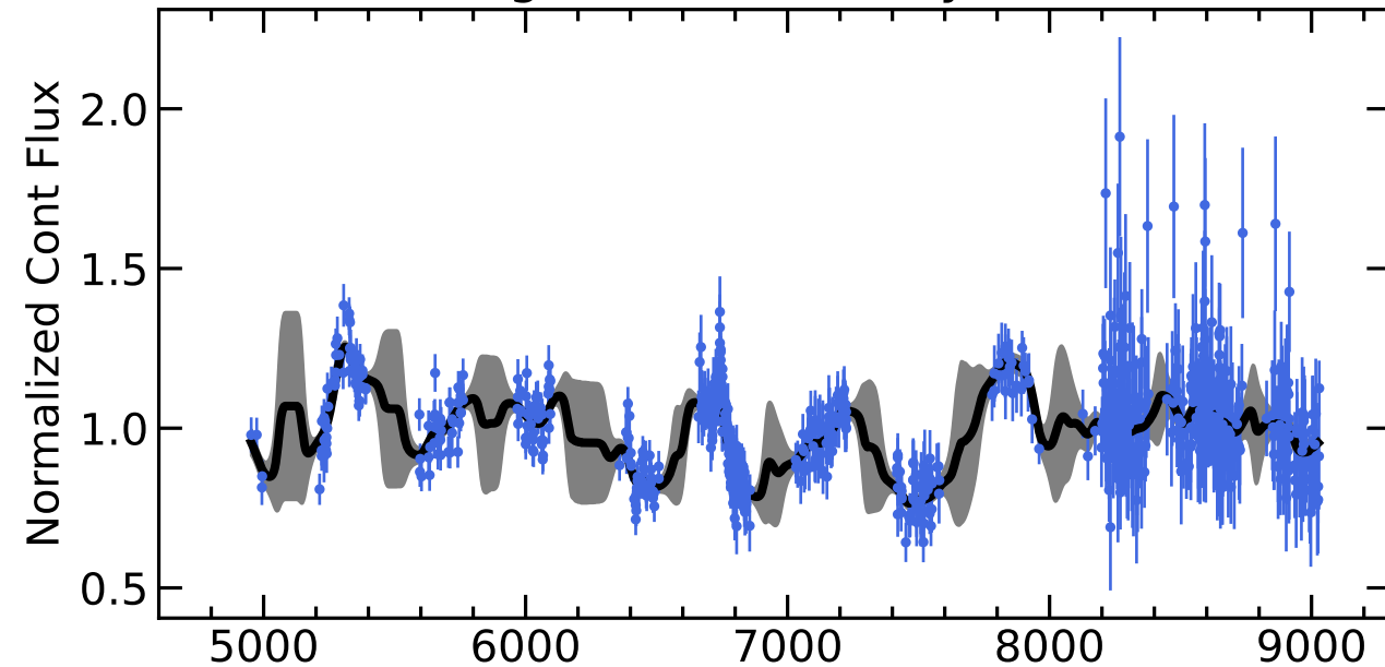
RM265 Light Curves (w/ PyROA model)
