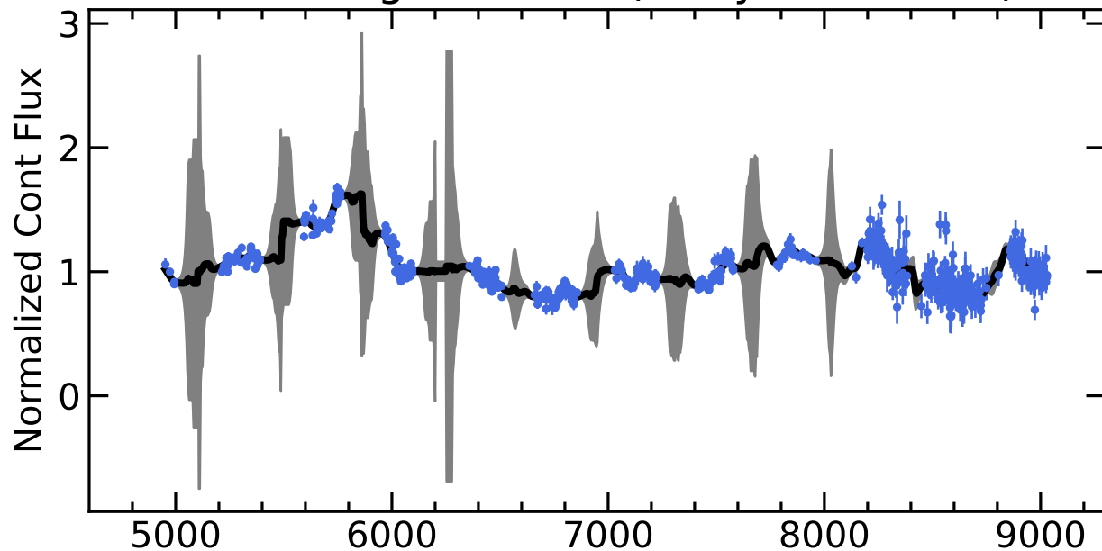
RM267 Light Curves (w/ PyROA model)
