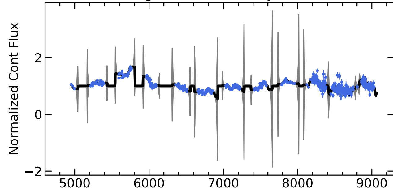
RM267 Light Curves (w/ PyROA model)
