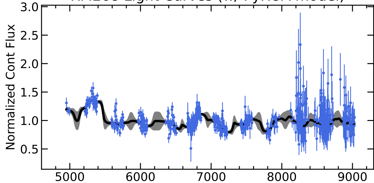
RM268 Light Curves (w/ PyROA model)
