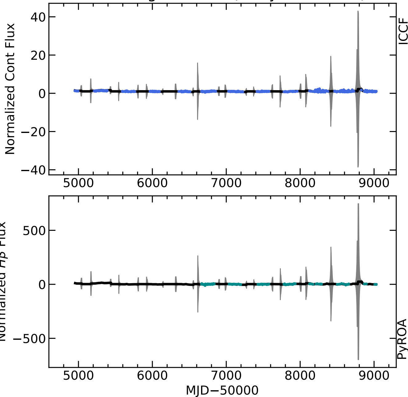
RM268 Light Curves (w/ PyROA model)
