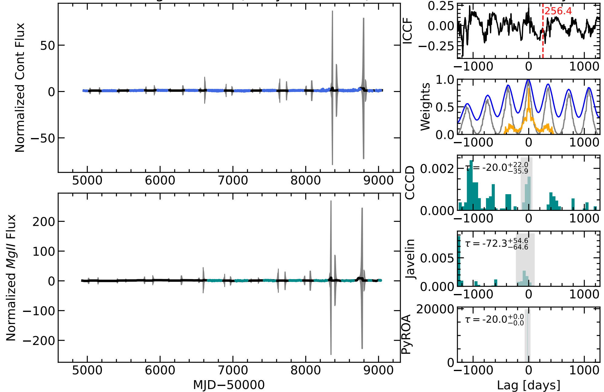
RM269 Light Curves (w/ PyROA model)
